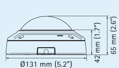
AXIS M3007-PV
