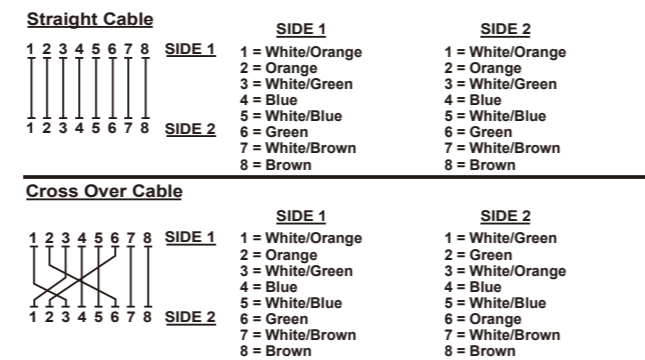
Figure A-1: Straight-Through and Crossover Cable
