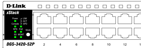
Figure 1- 12. LED indicators for the DGS-3420-52P
