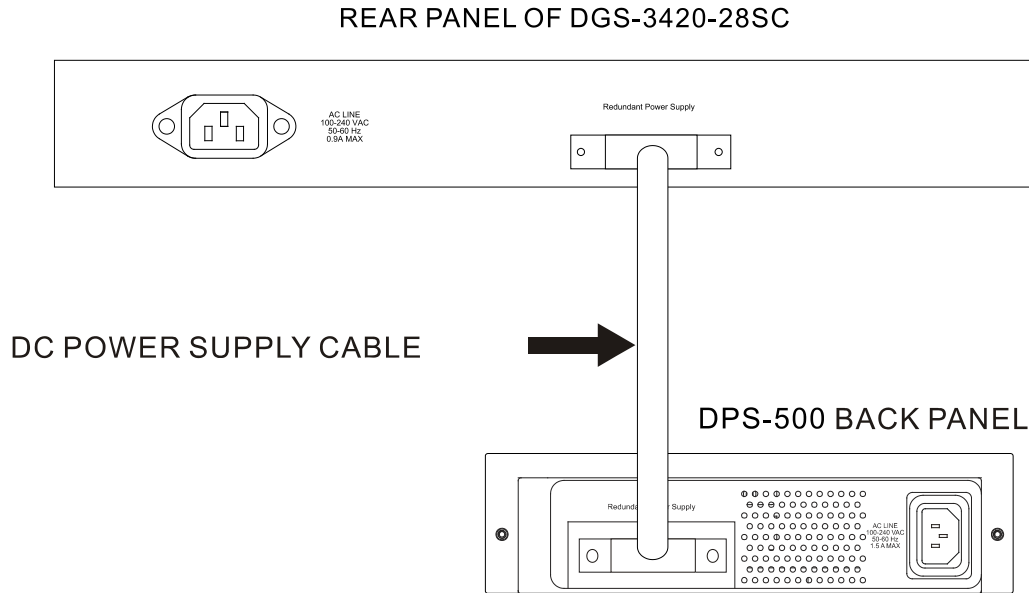
Figure 2–6 Connecting a DGS-3420 Series Switch to the DPS-500 (28TC, 28SC, 26SC, and 52T)
