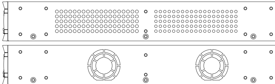
Figure 1- 20. Side panels of the DGS-3420-28TC Switch
