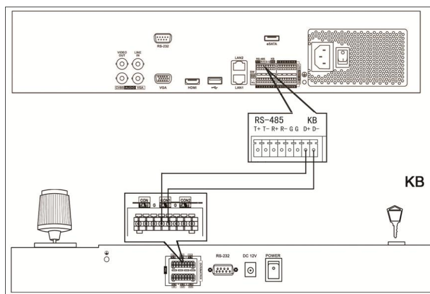
Figure 3-1 A Simple Connection between Keyboard and DVR
