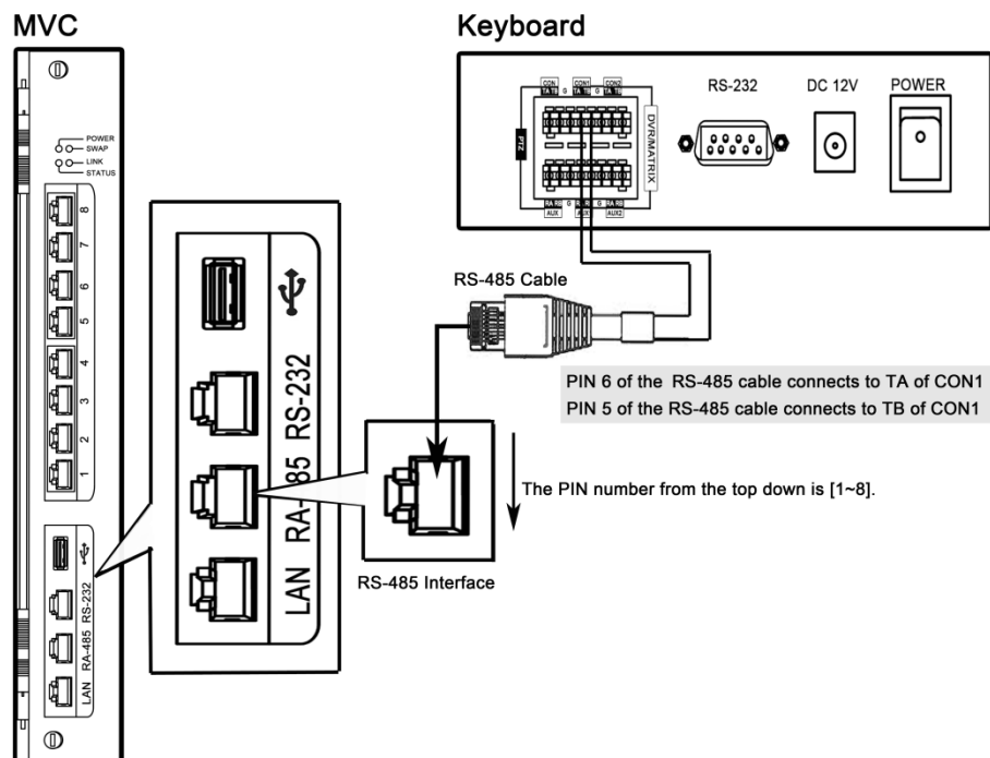
Figure 2-7 Connection between the keyboard and the VMS
