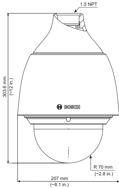
Dimensions in mm (inch)
