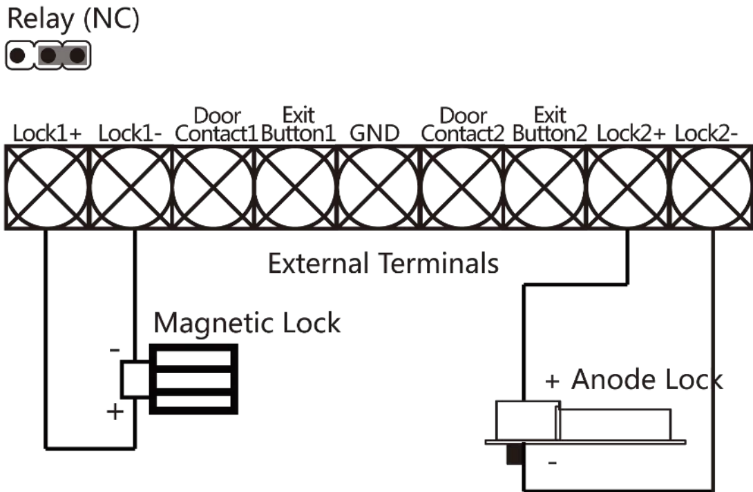
Figure 5-7 Wiring Diagram of Anode Lock
