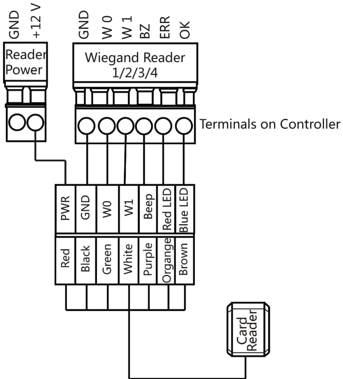
Figure 5-4 Wiegand Card Reader Wiring Diagram
