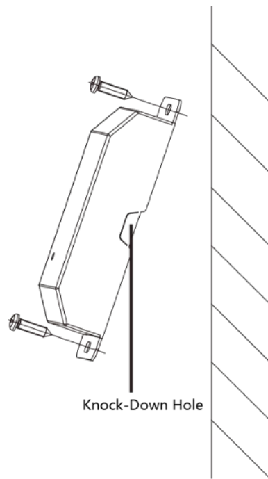
Figure 4-3 Install Secure Door Control Unit
