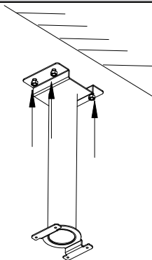
Figure 2-14 Fix Bracket
