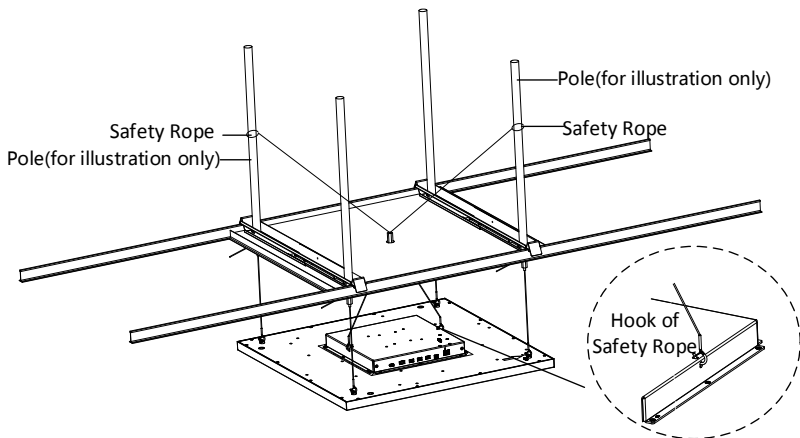
Figure 2-10 Install Safety Rope
