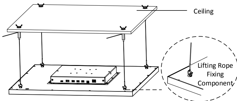
Figure 2-4 Fix Device and Lifting Rope
