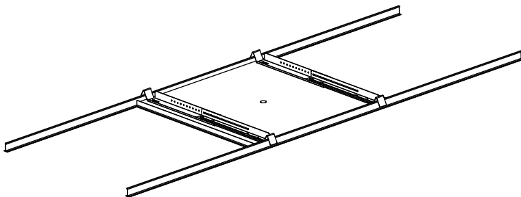
Figure 2-6 Fix Horizontal Pole Bracket and Lifting Rope Mounting Component
