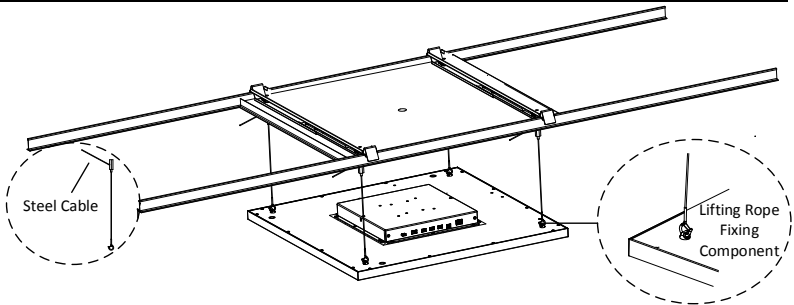
Figure 2-9 Fix Device and Lifting Rope
