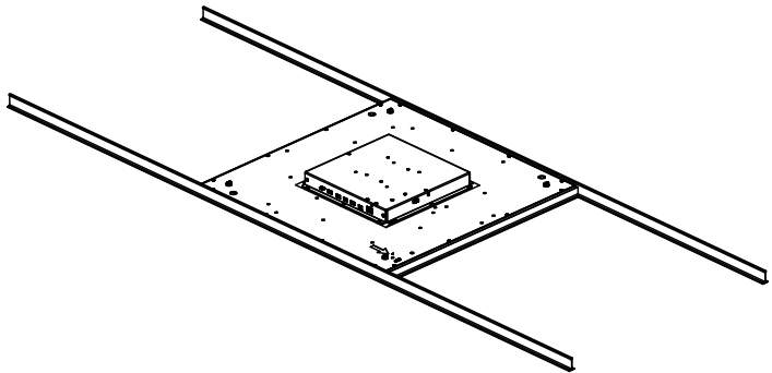
Figure 2-11 Place Device
