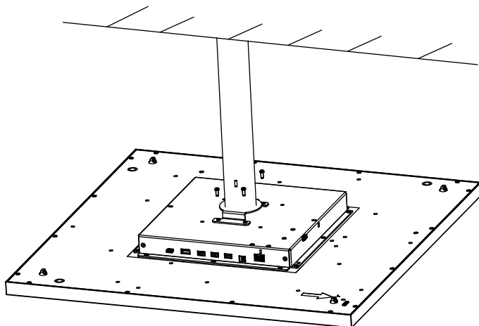
Figure 2-15 Fix Device
