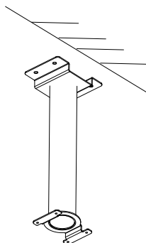
Figure 2-13 Drill Holes
