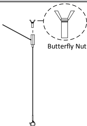
Figure 2-7 Remove Butterfly Nut
