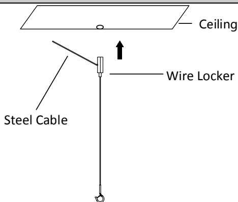
Figure 2-3 Fix Wire Locker
