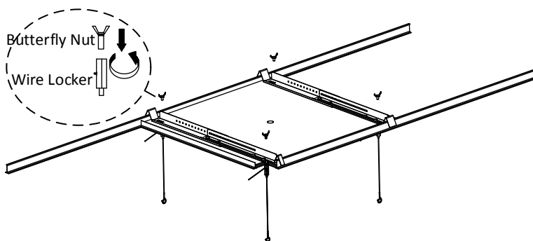
Figure 2-8 Fix Horizontal Pole Bracket and Wire Locker
