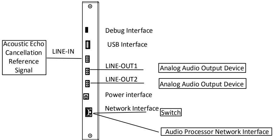
Figure 1-2 Interface
