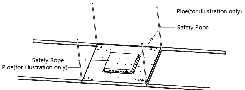
Figure 2-12 Install Safety Rope
