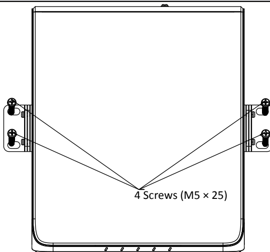
Figure 2-4 Fix Bracket
