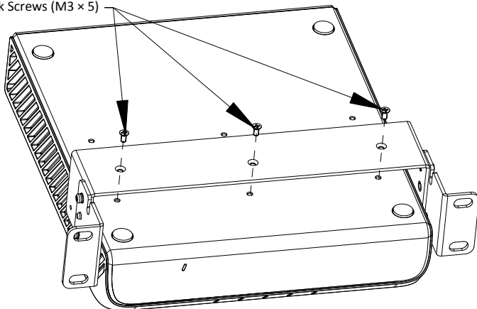
Figure 2-6 Fix Bracket to Device
