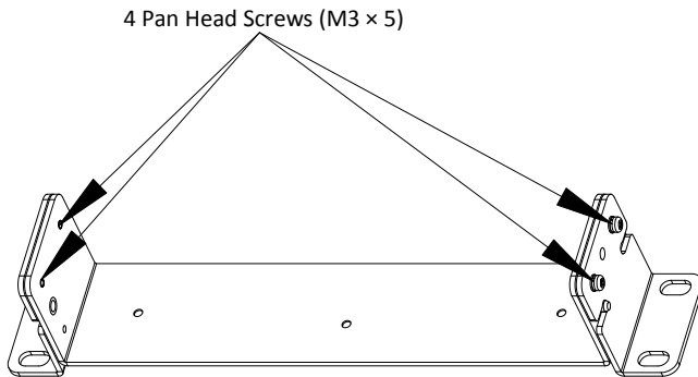
Figure 2-1 Assemble Bracket
