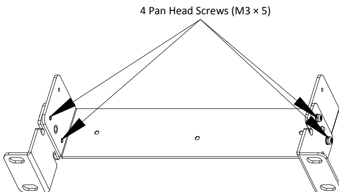
Figure 2-5 Assemble Bracket
