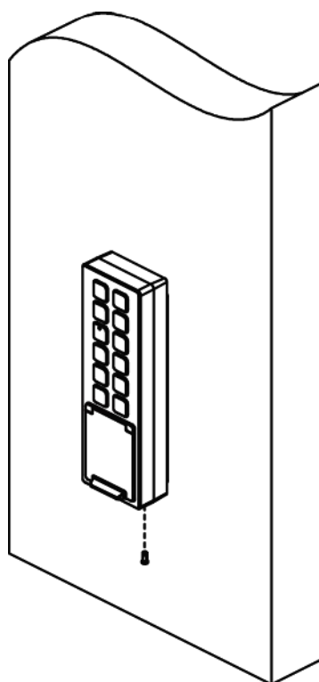
Figure 3-6 Secure Device
