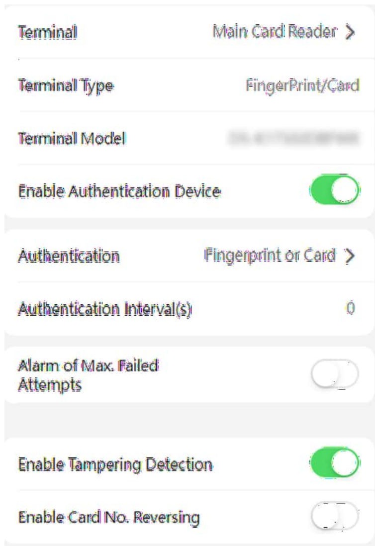
Figure 9-5 Authentication Settings
