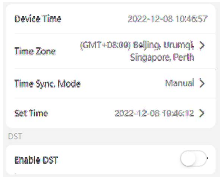
Figure 9-1 Time Settings
