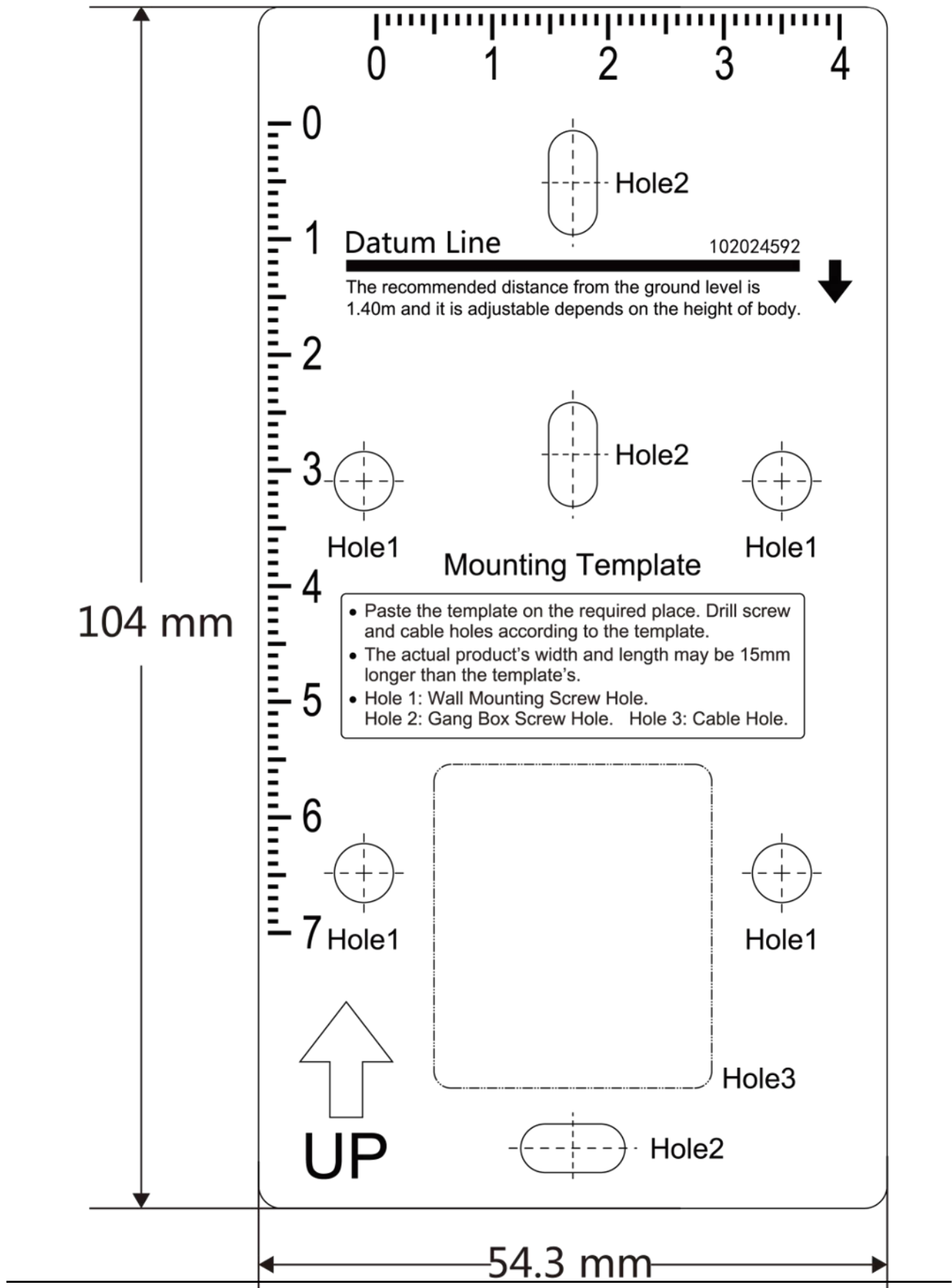
Figure 3-7 Mounting Template
