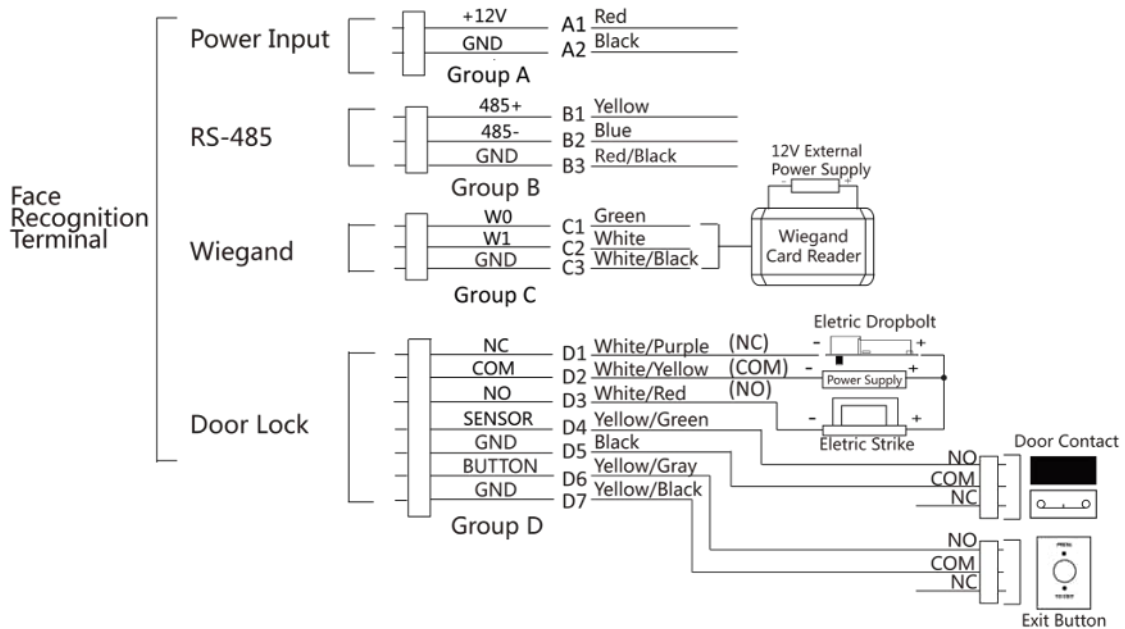
Figure 4-1 Device Wiring
