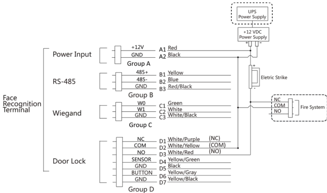
Figure 4-7 Device Wiring
