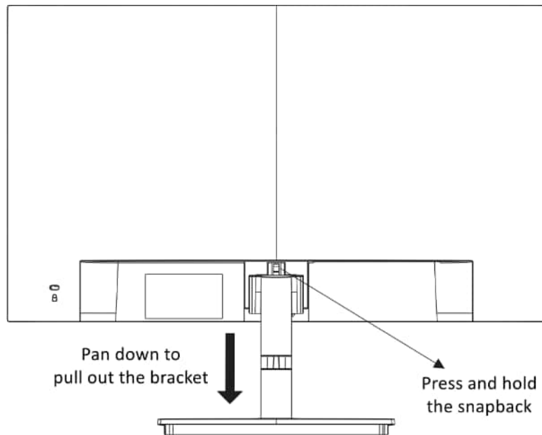
Figure 2-4 Remove the Device and Bracket
