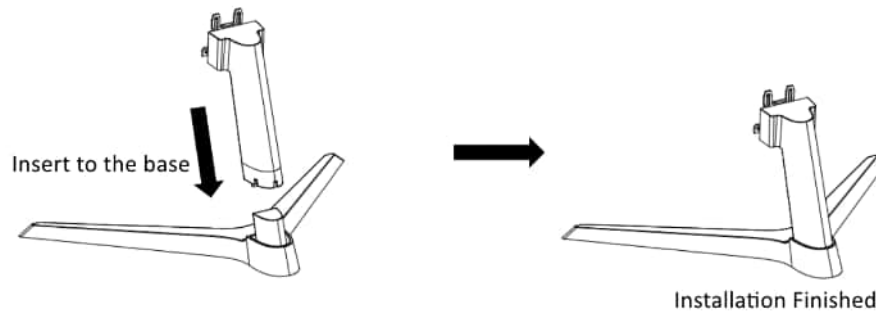
Figure 2-8 Install Bracket and Base (Model B)
