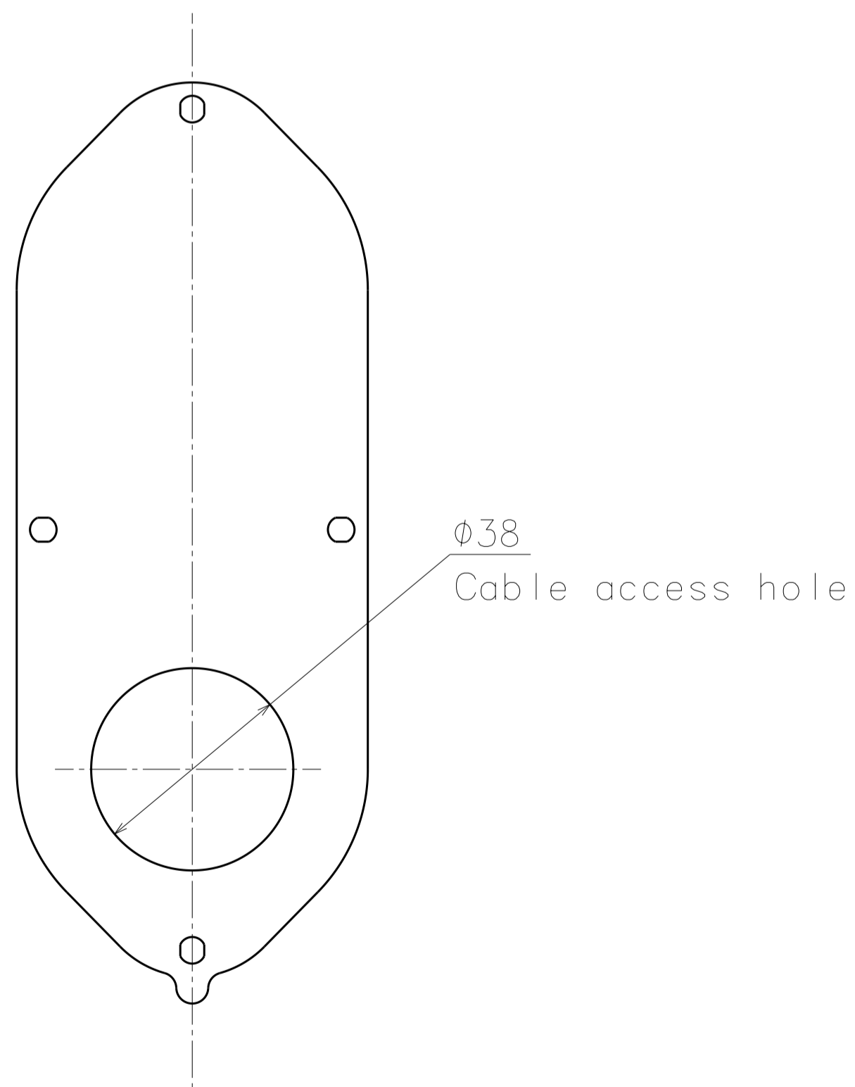
Plate (S=1:1)
