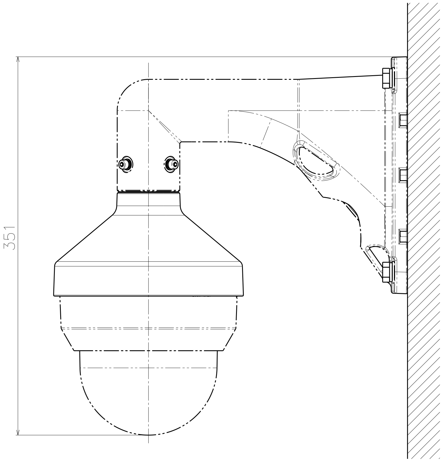
Attach to WV-S65301-Z1Sx & WV-QWL501S-W (S=1:2)
