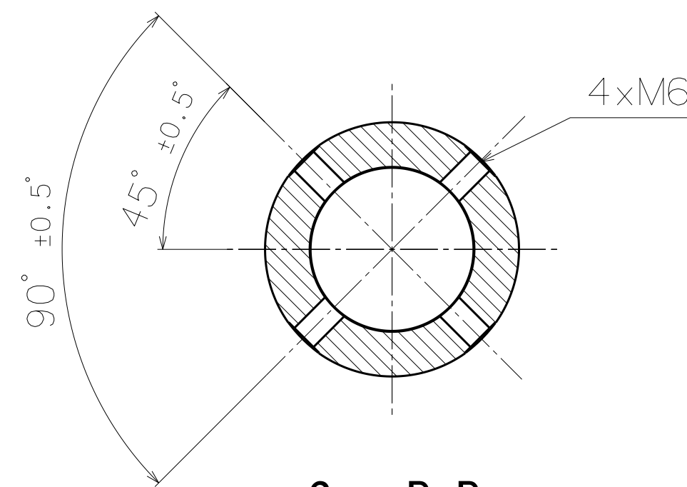
Sec B-B
