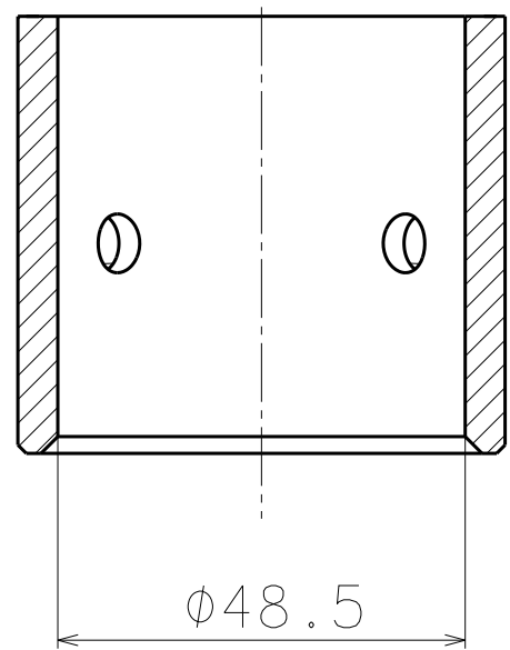
Sec B-B
