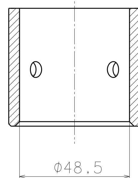
Sec B-B
