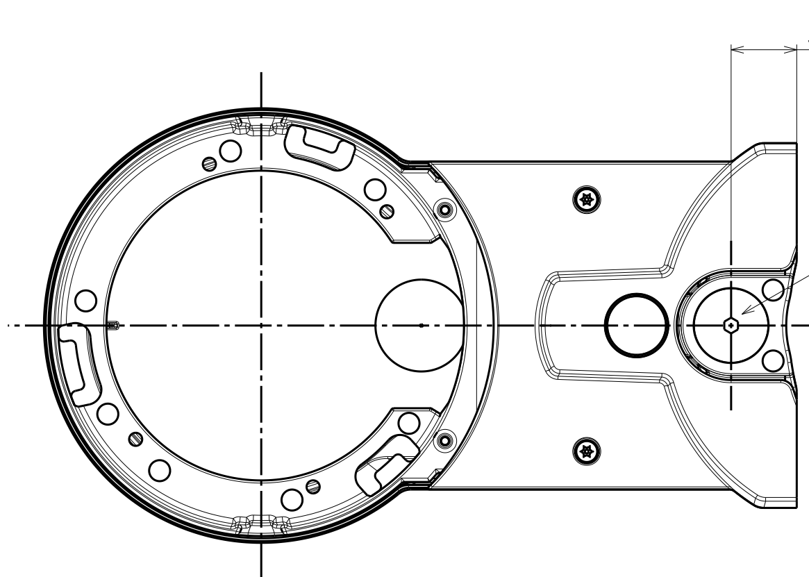
カメラ取付基準 Camera mounting standards
