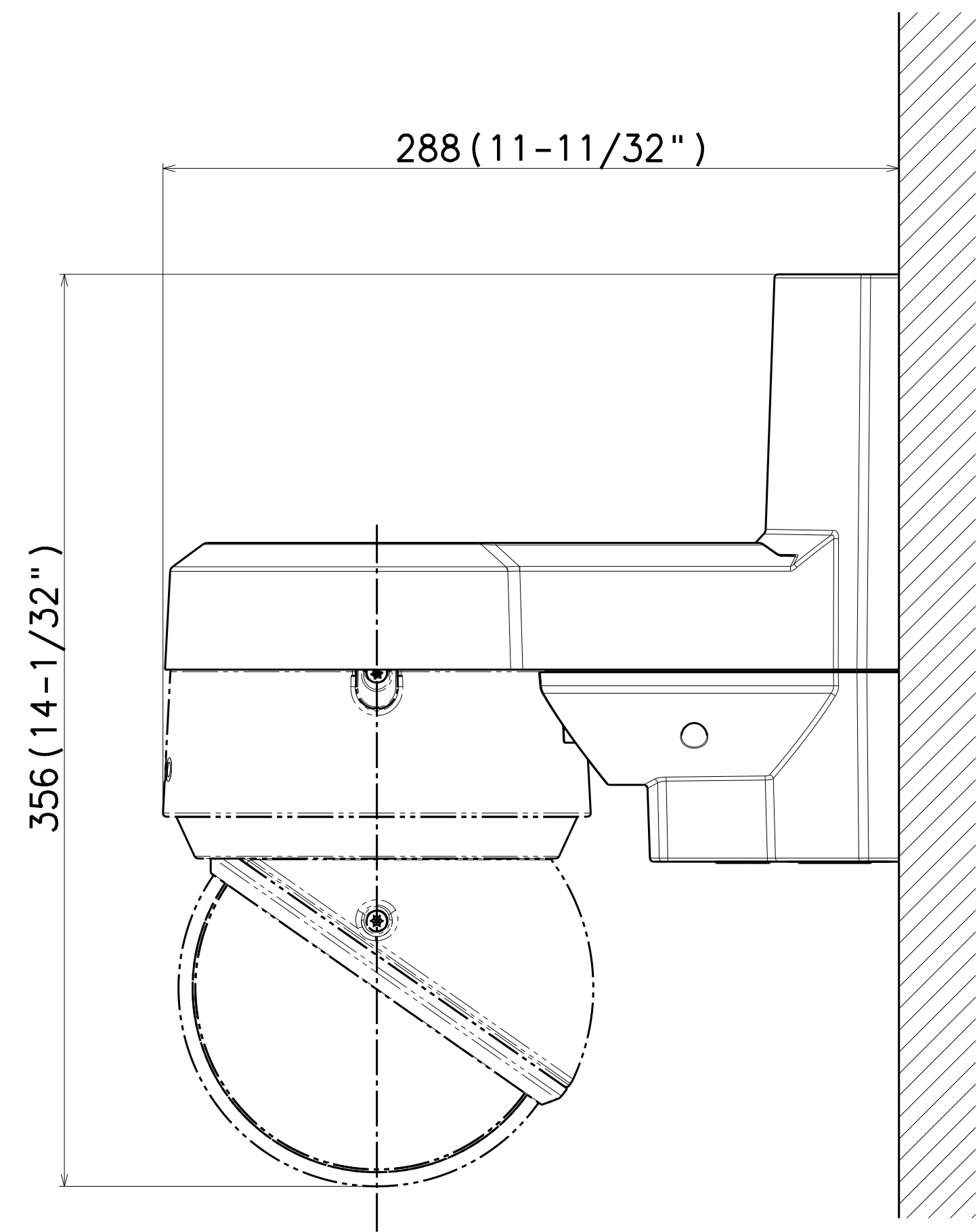
Wall mounting
