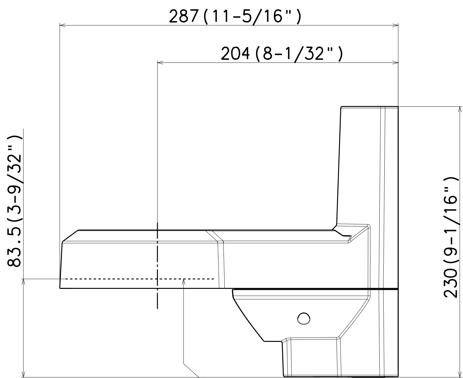
カメラ取付基準 Camera mounting standards
