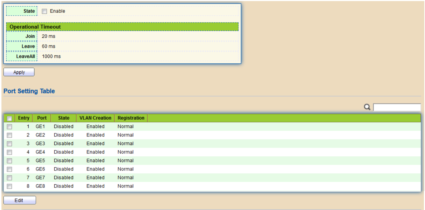
Figure 50 - VLAN > GVRP > Property
