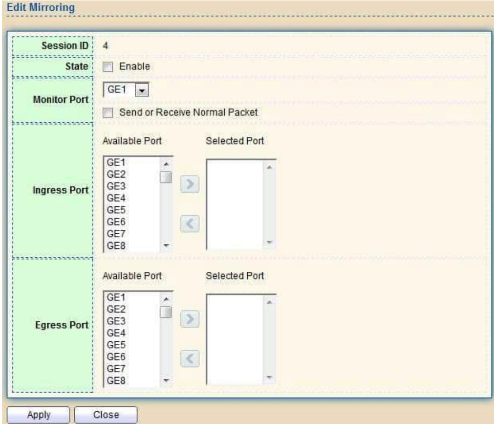
Figure 190 - Diagnostics > Mirroring > Edit Mirroring
