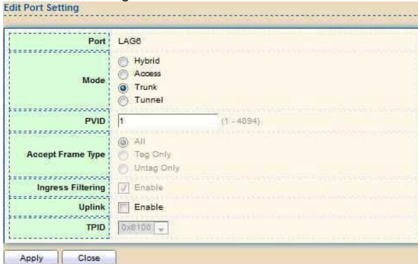
Figure 33 - VLAN > VLAN > Port Setting > Edit Port Setting
