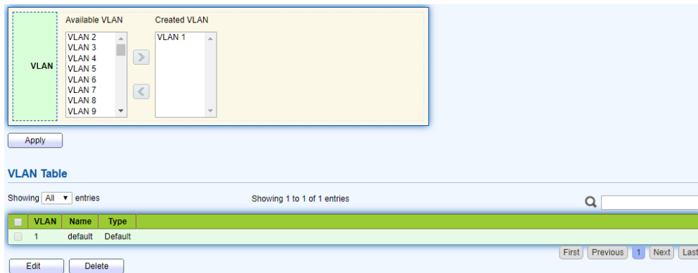
Figure 27 - VLAN > VLAN > Create VLAN
