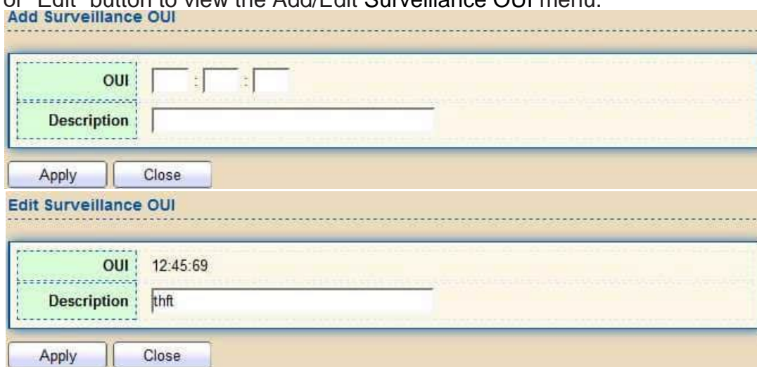
Figure 49 - VLAN > Surveillance VLAN > Surveillance OUI
