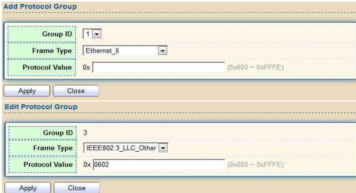
Figure 39 - VLAN > Protocol VLAN > Add/Edit Protocol Group
