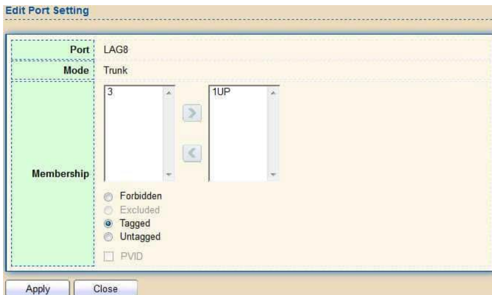
Figure 31 - VLAN > VLAN > Membership > Edit Port Setting
