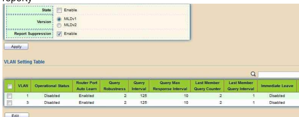
Figure 100 - Multicast > MLD snooping > Property
