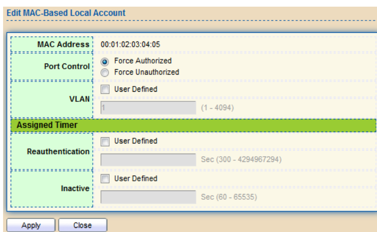
Figure 125 - Security > Authentication Manager > Add MAC-Based Local Account
